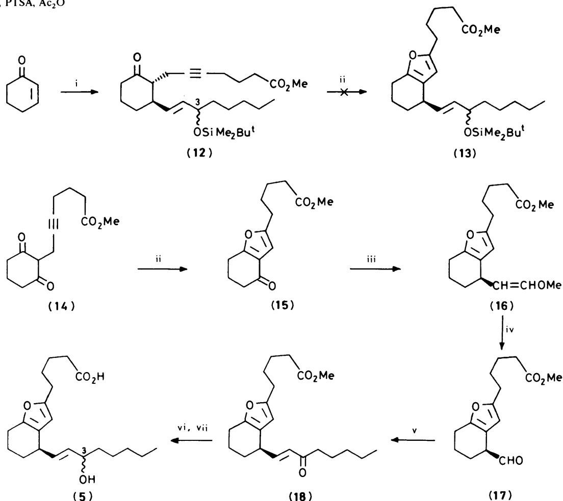
Scheme 1. Reagents: i, C 5 H 11 CH(OSiMe 2 Bu t )CH=CHCu(C≡CPr)Li then BrCH 2 C≡C[CH 2 ] 3 CO 2 Me; ii, PTSA, Ac 2 O; iii, Ph 3 P=CHOMe; iv, Me 3 SiI; v, (MeO) 2 P(O)CH(Na)COC 5 H 11 ; vi, NaBH 4 ; vii, NaOH
